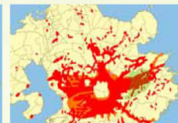
Volcanic explosion about 90,000 years ago
